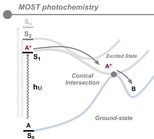
Fig. 3 Diagram of the photochemical step in the MOST cycle. Upon absorbing a photon, the stable isomer (A) reaches the excited state (A*) and subsequently returns to the ground state through decay, resulting in the formation of the metastable isomer (B).
