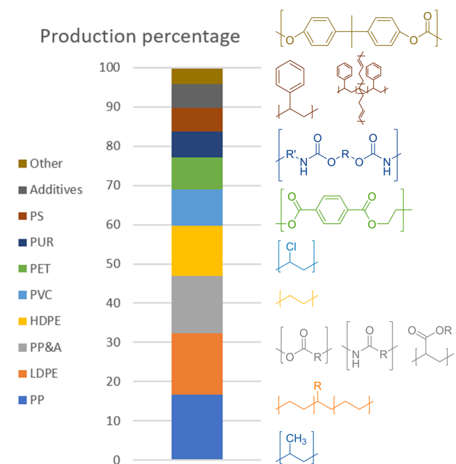
Scheme 2 Annual plastic production percentage (2015) with structures. 1
