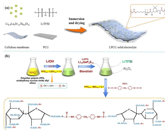
Fig. 6 (a) Schematic of the preparation of LPCU electrolyte; (b) the preparation process of PLL [(PU-LGPS)/Li + ] (ref. 47, copyrights 2023. Reproduced with permission from Elsevier. Ref. 12, copyrights 2022. Reproduced with permission from OAE Publishing Inc.).
