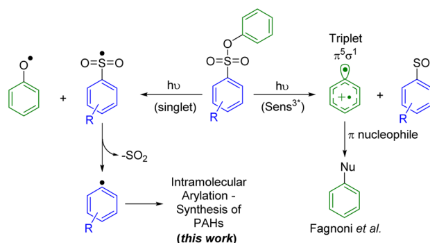
Fig. 1 Mechanistic pathways for the photocleavage of the phenylsulfonate moiety.
