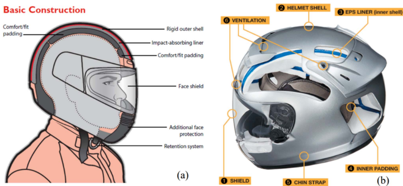
Fig. 7 Schematic diagrams showing the various components in a (a) typical motorcycle helmet and (b) a Shoei motorcycle helmet. 71
