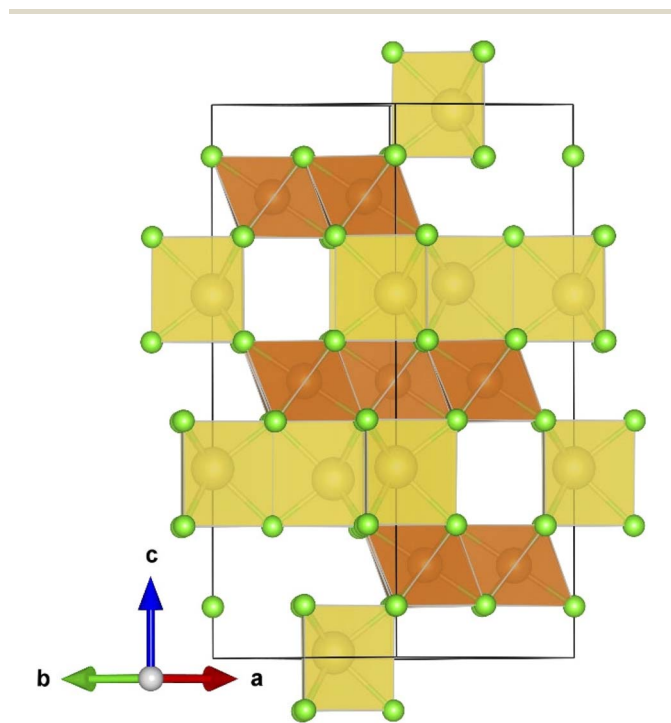
Fig. 1 Hexagonal representation of the \text{Na}_2\text{Mg}_3\text{Cl}_8 lattice structure ( R\bar{3}m space group). Yellow prisms represent the [\text{NaCl}] polyhedron, light brown the [\text{MgCl}_6] octahedron and green balls \text{Cl}^- ions.
