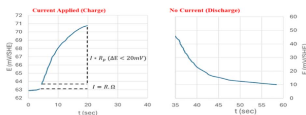
Fig. 12 A graph illustrating the GP measurement of the anodic direction with a 50 \mu A injection over 30 s, revealing the change in \Delta E over time throughout the charge and discharge phases. 34
