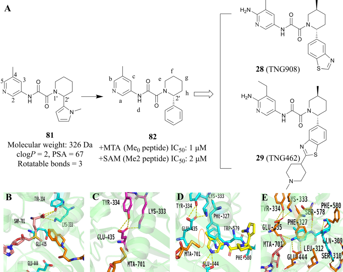
Fig. 11 The development strategy, which combined the HTS and SBDD methodologies, yielded the 28 (TNG908). 85,86 (A) The development route of 28 (TNG908) and 29 (TNG462). (B) X-ray cocystal structure of PRMT5/SAM/substrate complex. Glu435 rotates toward substrate side chain (PDB 4X61). 21,22 (C) X-ray cocystal structure of PRMT5/MTA complex. Glu435 rotates to fill space previously filled by SAM (PDB 8VEO). 21,22,85 (D) X-ray cocystal structure of 82R (yellow) bound to PRMT5/MTA (PDB 8VET). 85 (E) X-ray cocystal structure of 28 (TNG908) bound to PRMT5/MTA (PDB 8VEY). 85
