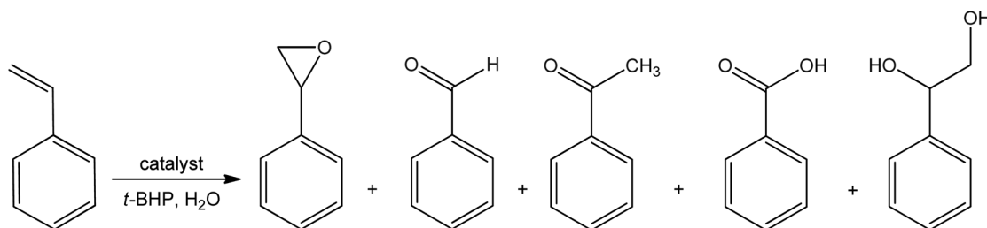
Fig. 5 Catalytic oxidation of styrene by oxovanadium(V) complexes.
