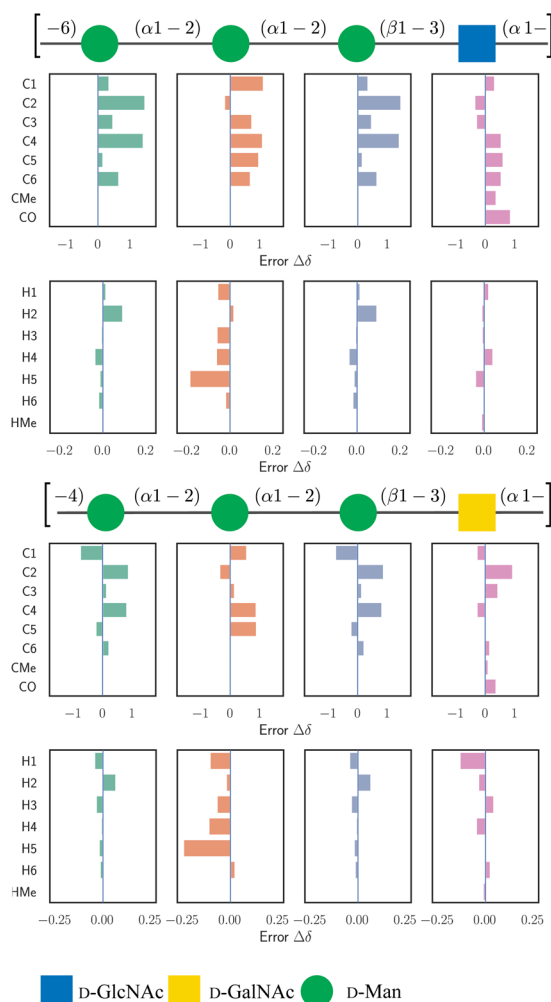
Fig. 10 The figure illustrates the prediction errors for the 13 C and 1 H chemical shifts of two E. coli O-antigen polysaccharides, each composed of tetrasaccharide repeating units, from serogroup O77 (upper) and serogroup O176 (lower). 27,28 The structures are visualized using symbols from the SNFG standard. 29 The repeating units are enclosed in square brackets. The box plots visually represent the prediction errors Δδ per-atom basis.
