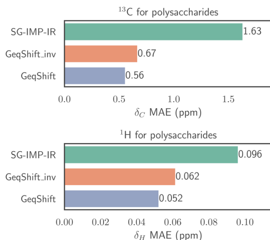
Fig. 9 Prediction performance for chemical shifts ( 13 C and 1 H) in terms of mean absolute error (MAE) within the context of the two polysaccharides introduced in Fig. 10. In this evaluation, the models employ an average prediction derived from the ten models trained during ten-fold cross-validation.
