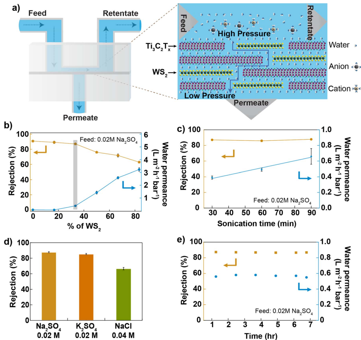
Fig. 2 Ti_3C_2T_x + WS_2 composite membrane's test in cross-flow systems; (a) Illustration of Ti_3C_2T_x + WS_2 composite membrane in the cross-flow cell. (b) Performance of Ti_3C_2T_x + WS_2 composite membrane based on WS_2 content, Ti_3C_2T_x was sonicated for 30 min. (c) Performance of Ti_3C_2T_x + WS_2 composite membrane by varying sonication time of Ti_3C_2T_x nanosheets. (d) Salt rejection of Ti_3C_2T_x + WS_2 composite membrane for different salts (each salt at 0.02 M concentration). (e) Stability test of Ti_3C_2T_x + WS_2 composite membrane for up to 7 hours. In each figure, error bars represent standard deviations from >3 replicates.
