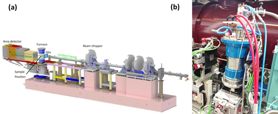
Fig. 2 (a) The layout of the Spatz neutron beam instrument with furnace installed on the neutron beamline at the Australian Nuclear Science and Technology Organization (ANSTO), recreated from ref. 21 under creative commons licence CC BY 4.0 DEED. Green arrow indicates the neutron beam path. (b) Photograph of the furnace installed on the neutron beamline for EG synthesis and in situ monitoring using neutron reflectometry at ANSTO.
