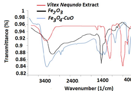
Fig. 2 FTIR spectrum of the VN-Fe_3O_4-CuO nanocatalyst.
