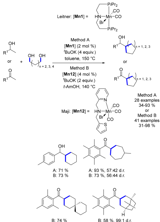
Scheme 62 Synthesis of cycloalkanes using di-alkylation of ketones and secondary alcohols, as reported by Leitner and Maji.
