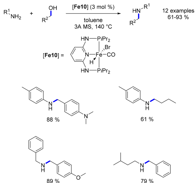
Scheme 29 Alkylation of amines.
