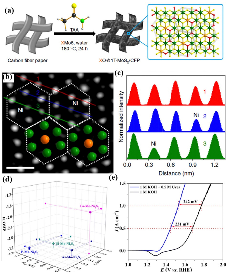
Fig. 11 (a) The preparation process of \text{XO}@1\text{T-MoS}_2/\text{CFP} ; (b) aberration-corrected atomic resolution HAADF-STEM image (scale bar: 0.5 nm); (c) intensity profiles along the lines indicated in (b). 133 Copyright 2019, Springer Nature. (d) A comparison of E_{\text{ads}}(\text{urea}) , \epsilon_d , and ICOHP values. (e) A comparison of the UOR and OER activity of \text{P-Mo-Ni}_3\text{S}_2/\text{NF} . 135 Copyright 2023, Royal Society of Chemistry (RSC).
