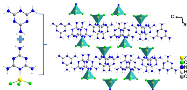
Fig. 8 Crystal structure of (\text{H}_7\text{C}_3\text{N}_6)(\text{H}_6\text{C}_3\text{N}_6)\text{ZnCl}_3 .
