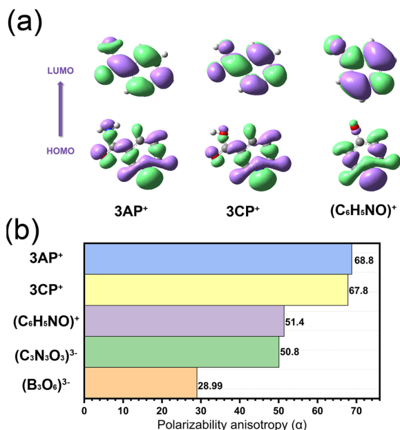
Scheme 1 The HOMO and LUMO maps (a) as well as polarizability anisotropy (b) of related units.
