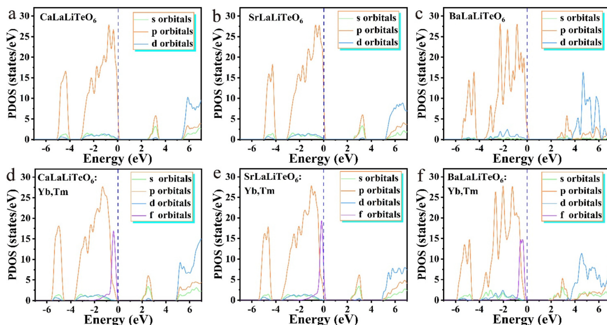
Fig. 5 The PDOS, bonding and anti-bonding orbitals of (a–c) ALaLiTeO 6 and (d–f) ALaLiTeO 6 :Yb,Tm with (A = Ca, Sr, and Ba).
