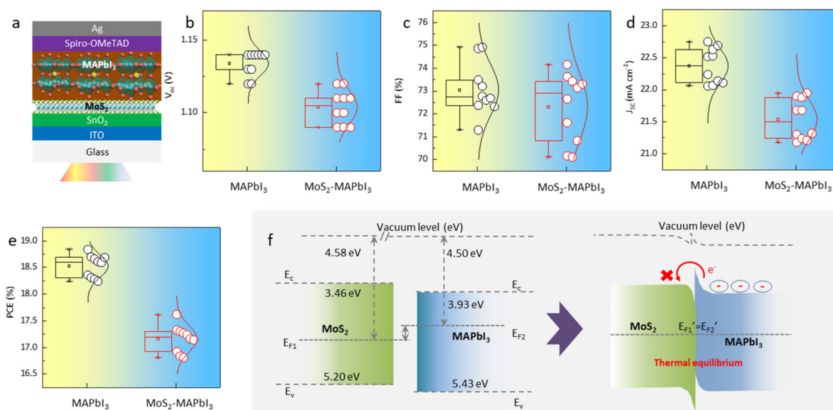
Fig. 4 Bandgap alignment between MoS 2 and MAPbI 3 . (a) Schematic structure of the MoS 2 -MAPbI 3 device. (b–e) Distribution of V OC , J SC , FF, and PCE values collected from 10 MAPbI 3 and 10 MoS 2 -MAPbI 3 devices. (f) Energy level change scheme of MoS 2 and MAPbI 3 .
