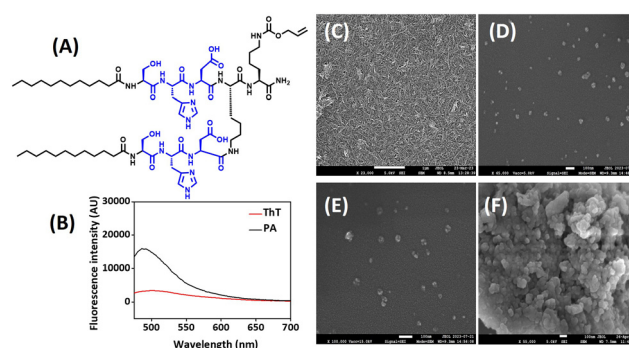
Fig. 1 (A) Structure of self-assembled, branched peptide amphiphile (PA). (B) ThT assay. (C–F) FESEM images of: (C) PA, (D) CeNP, (E) TC, and (F) TCP. Scale bar: (C) 1 \mu m, and (D–F) 100 nm.
