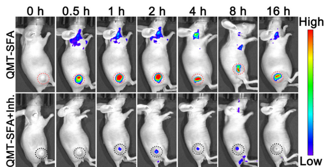
Fig. 4 Time-course fluorescence images of 4T1 tumor-bearing mice after the intratumoral injection of 0.25 \text{mg kg}^{-1} QMT-SFA. For the “QMT-SFA + Inh.” group, tumors were pretreated with 0.02 \text{mg kg}^{-1} inhibitor for 0.5 h before QMT-SFA injection. The dashed circles indicate tumor regions.
