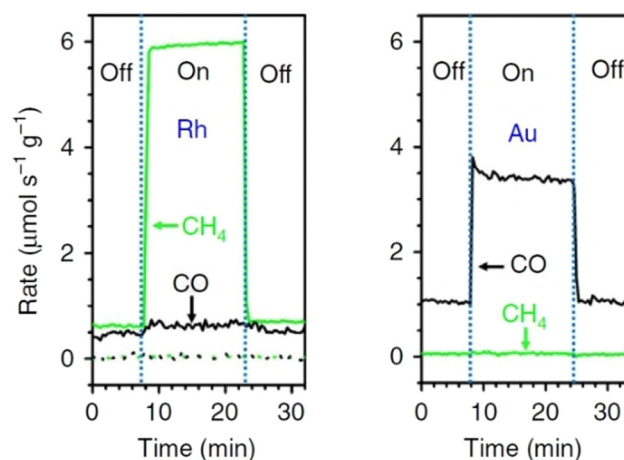
Fig. 15 Rates of production of CH_4 (green) and CO (black) at 623 K on Rh/Al_2O_3 (solid lines) and Al_2O_3 (dotted lines) under UV illumination and dark conditions (light intensity – 3 W cm -2 ). CH_4 production and selectively is greatly enhanced by ultraviolet light on Rh/Al_2O_3 . Rates of production of CO (black) and CH_4 (green) at 623 K on Au/Al_2O_3 visible illumination and under dark conditions (light intensity – 3 W cm -2 ). "Reproduced from ref. 96 with permission from Springer Nature, copyright 2017".
