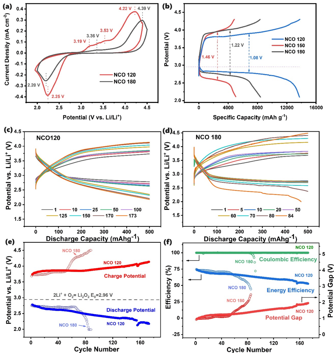
Fig. 4 (a) CV analysis @ 0.2 \text{ mV s}^{-1} and (b) full discharge–charge @ 100 \text{ mA g}^{-1} , and selected discharge–charge curves of (c) NCO 120 and (d) NCO 180 cathode-based LABs operated at 100 \text{ mA g}^{-1} for a limited capacity of 500 \text{ mA h g}^{-1} . (e and f) Cycle life and performance analysis of LABs with NCO 120 and NCO 180 based cathodes with cut-off discharge capacity of 500 \text{ mA h g}^{-1} with 1 \text{ M LiTFSI} dissolved in TEGDME electrolyte.
