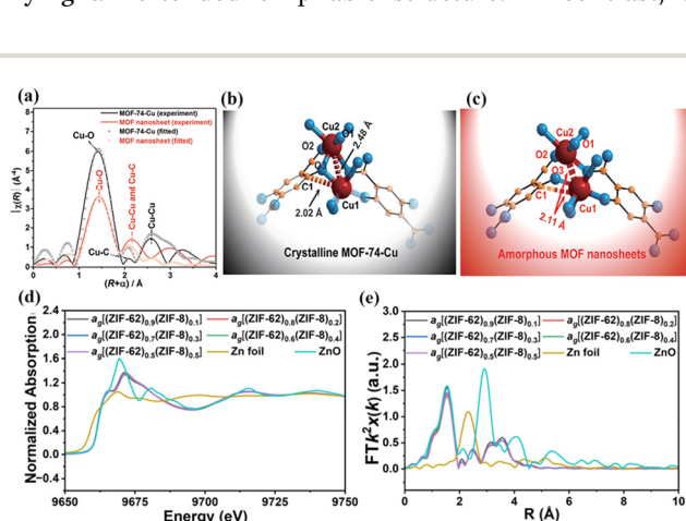
Fig. 4 (a) EXAFS spectra of MOF crystals and nanosheets. Suggested structures of (b) MOF crystals and (c) nanosheets deduced from the analysis of EXAFS. Reproduced with authorisation from ref. 54 and copyright 2021 by The Royal Society of Chemistry. (d) Normalized XANES spectra and (e) EXAFS R-plots of MOF CGC membranes. Reproduced with authorisation from ref. 45 and copyright 2023 by Wiley-VCH GmbH.
