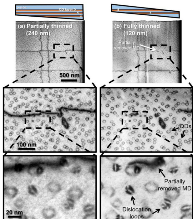
Fig. 4 (a) [001]-zone plan-view BF STEM of the partially thinned sample from the no-TL laser. Magnified insets show a dislocation loop cluster near a climbed MD. The inset diagram above is a side profile showing approximately which of the five QD layers remain in the thinned sample. (b) The same sample thinned further to partially remove the MD on the p side of the laser, but not the QDs themselves. Notably, the dislocation loops that form near this MD all remain behind indicating the loops are centered not around the MD but around the QDs themselves.
