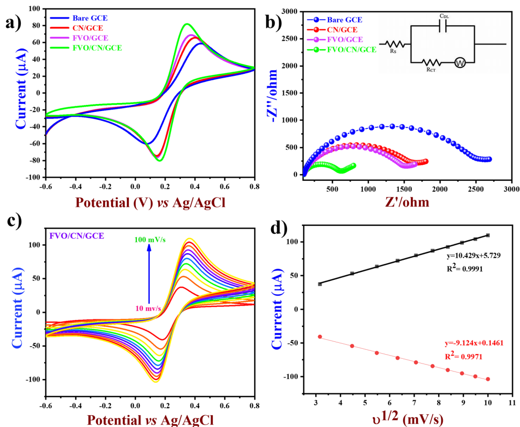
Fig. 4 (a) CV plots and (b) EIS plots of bare and different modified electrodes with 0.1 M KCl in 5 mM Fe(CN) 6 3-/4- , (c) CV plots with increase in the scan rate from 10 to 100 mV s -1 and (d) linear plots of I_{pa} and I_{pc} vs. square roots of scan rates of FVO/CN/GCE with 0.1 M KCl in 5 mM Fe(CN) 6 3-/4- .
