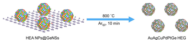
Scheme 1 A pictorial representation of the formation of high-entropy germanide (HEG: AuAgCuPdPtGe) from high-entropy alloy nanoparticles decorated germanane (HEA NPs@GeNSs). HEA NPs@GeNSs were rapid annealed at 800 °C under Ar flow for 10 minutes. The products were collected after rapidly cooling to room temperature. (Note: for clarity, hydrogen atoms on the germanane surfaces are not shown.)
