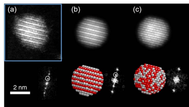
Fig. 7 (a) STEM-HAADF image of one Ag/Pt NP oriented along the [011] zone axis showing L1 phase with alternating planes of Ag and Pt and its corresponding FFT showing the superstructure reflections (marked with white circle). In the HAADF image, Pt atom columns are brighter than Ag atom columns, for Pt has a higher atomic number than Ag. (b and c) Simulated STEM-HAADF images along [011] zone axis for an L1 structure and a random solid solution, respectively. Adapted from ref. 97 under CC BY license @ 2019, the Author(s). Copyright 2019, Springer Nature.
