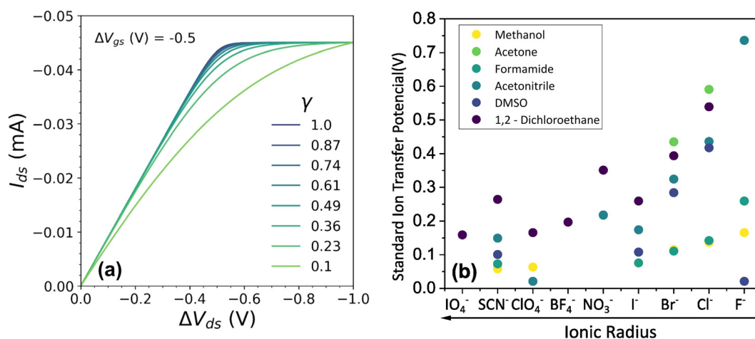
Fig. 4 (a) Effect of \gamma variation on output curve shape. Here were used the following parameters w = 1.5 mm, h = 100 nm, l = 250 \mu m, \sigma = 1.5 S \text{cm}^{-1} , \sigma_{\text{res}} = 1 \times 10^{-4} S \text{cm}^{-1} , \mathcal{E}_{\text{pol}}^{\ominus'} = 0 V, T = 298.15 K, \Delta V_{\text{gs}} = -0.5 V. (b) Standard Ion Transfer Potential for anions from water to organic solvent from ref. 66–68 with adaptations.
