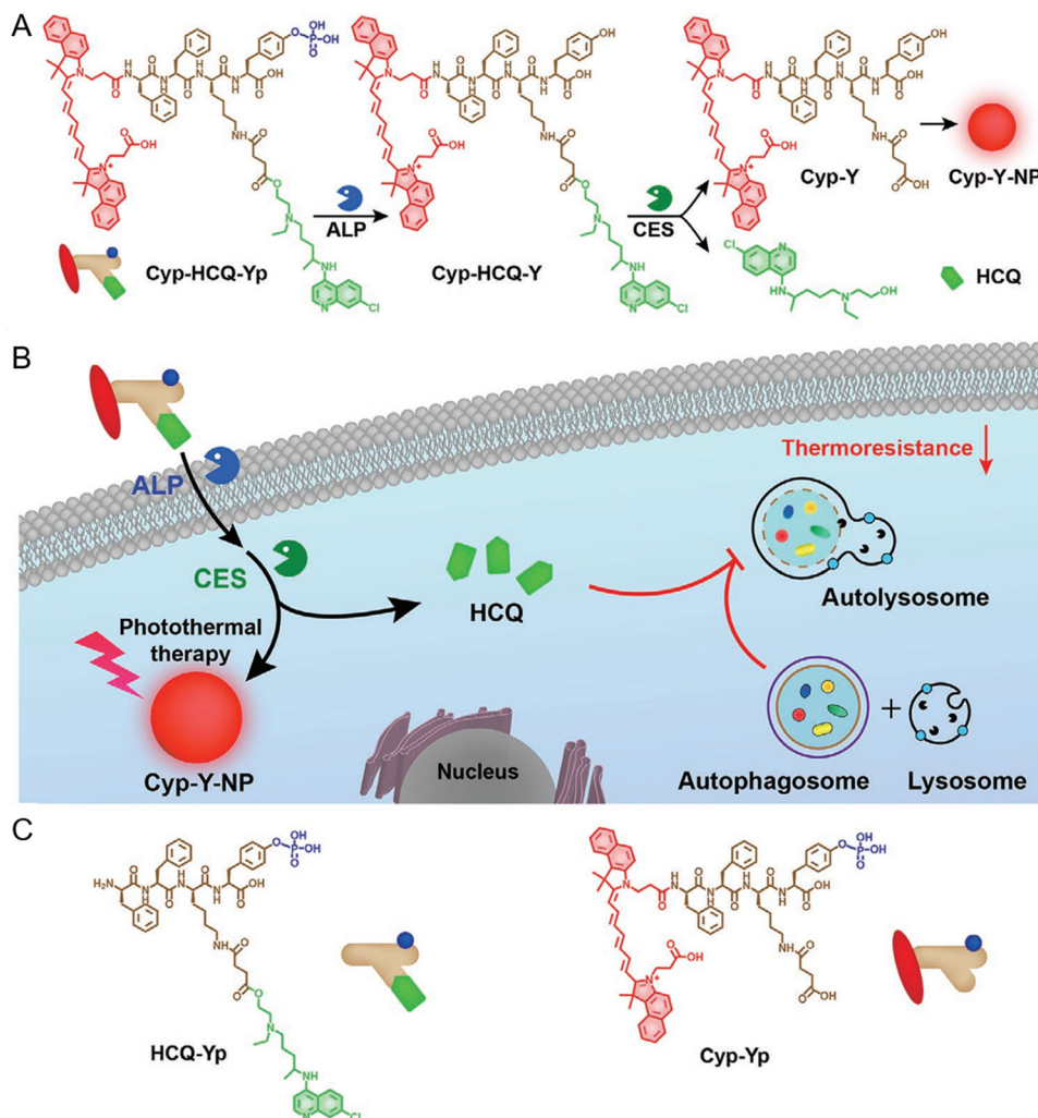
Fig. 9 A "smart" prodrug Cyp-HCQ-Yp for autophagy-inhibited mild-temperature photothermal therapy. (A) The enzymatic transformation of Cyp-HCQ-Yp into Cyp-Y which self-assembles into Cyp-Y-NPs. (B) Schematic of the working mechanism of Cyp-HCQ-Yp. (C) Chemical structures of two control agents HCQ-Yp and Cyp-Yp. Reproduced from reference 105 with permission from Wiley, copyright 2021.
