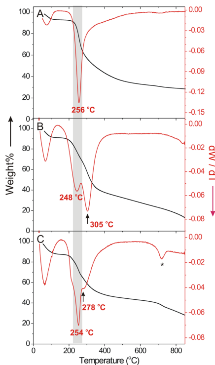
Fig. 4 TGA thermogram and differential thermogravimetric (DTG) curves of (A) glycated CS, (B) Glc-ECS, and (C) Glc-ECS/Cu. Asterisk at 718 °C indicates the decomposition of residual sulfate ions from CuSO 4 .
