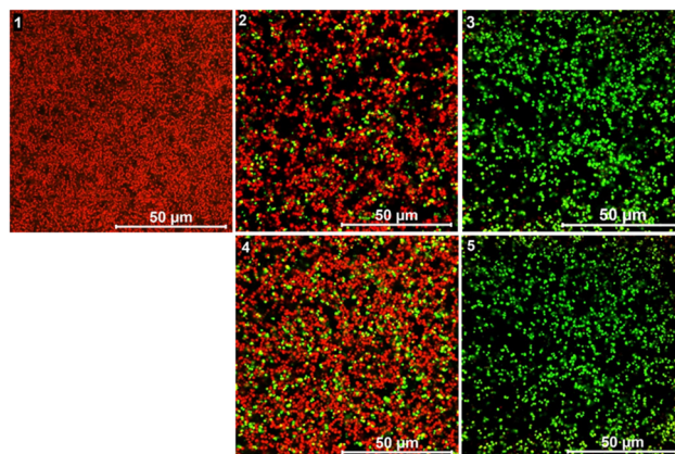
Fig. 4 2D confocal images of the biofilm population of P. aeruginosa where red = live cells and green = dead cells. (1) Growth control; (2) biofilm treated with 0.025 \times MBEC of TMC-S1; (3) biofilm treated with 0.5 \times MBEC of TMC-S1; (4) biofilm treated with 0.025 \times MBEC of TMC-S2 and (5) biofilm treated with 0.5 \times MBEC of TMC-S2.
