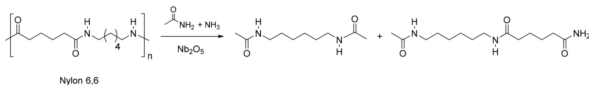
Fig. 13 Sketch of transamidation reaction of nylon 6,6 over heterogeneous Nb 2 O 5 catalyst.
