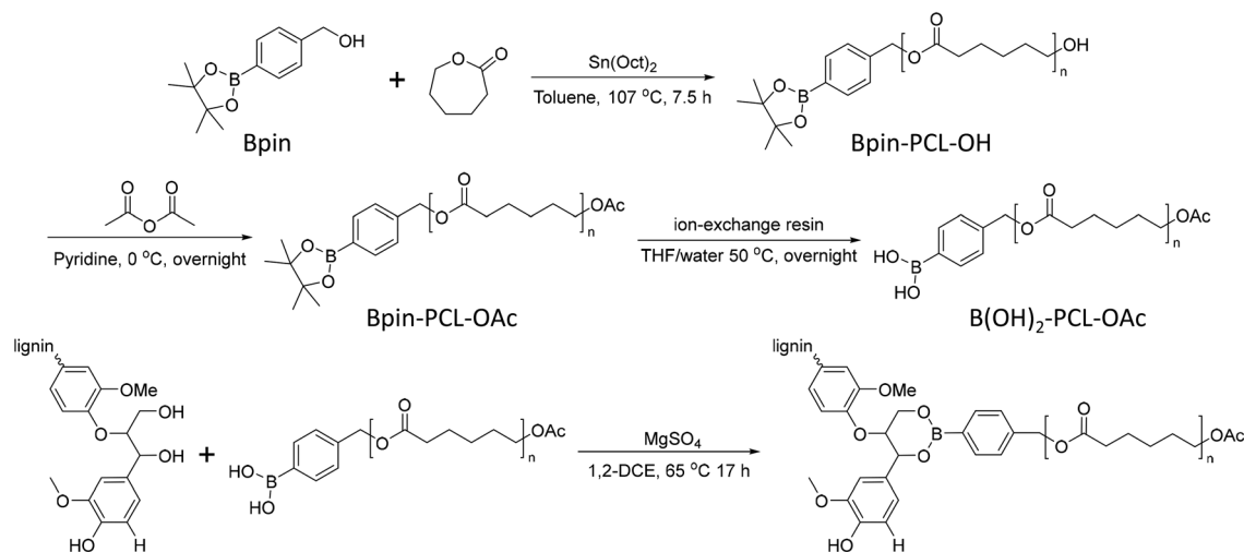
Scheme 11 Synthesis of separately prepared PCL and graft copolymerization of PCL onto lignin. Terminal \beta\text{-O-4} softwood lignin unit is used for simplicity.
