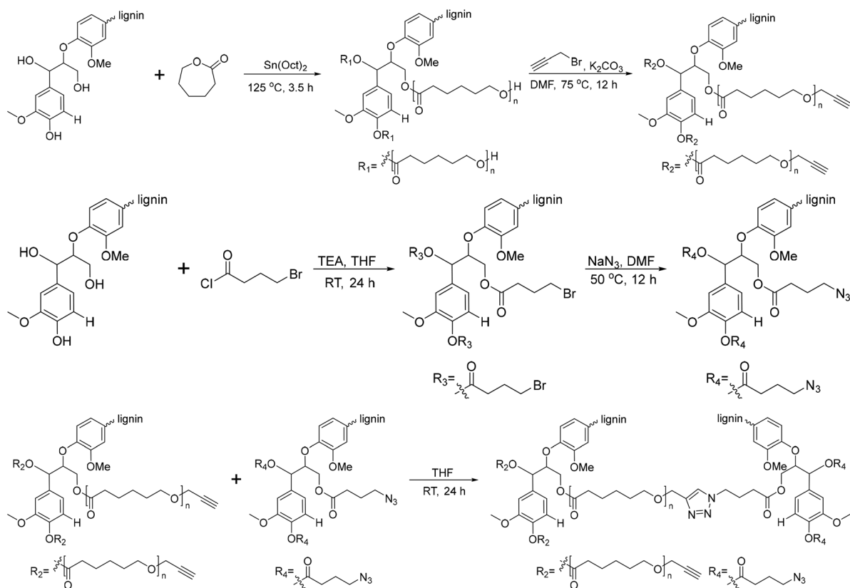
Scheme 12 Synthesis of lignin-graft-PCL by the graft-from method and lignin-graft-PCL-graft-lignin by the graft-onto method. Terminal \beta\text{-O-4} softwood lignin unit is used for simplicity.
