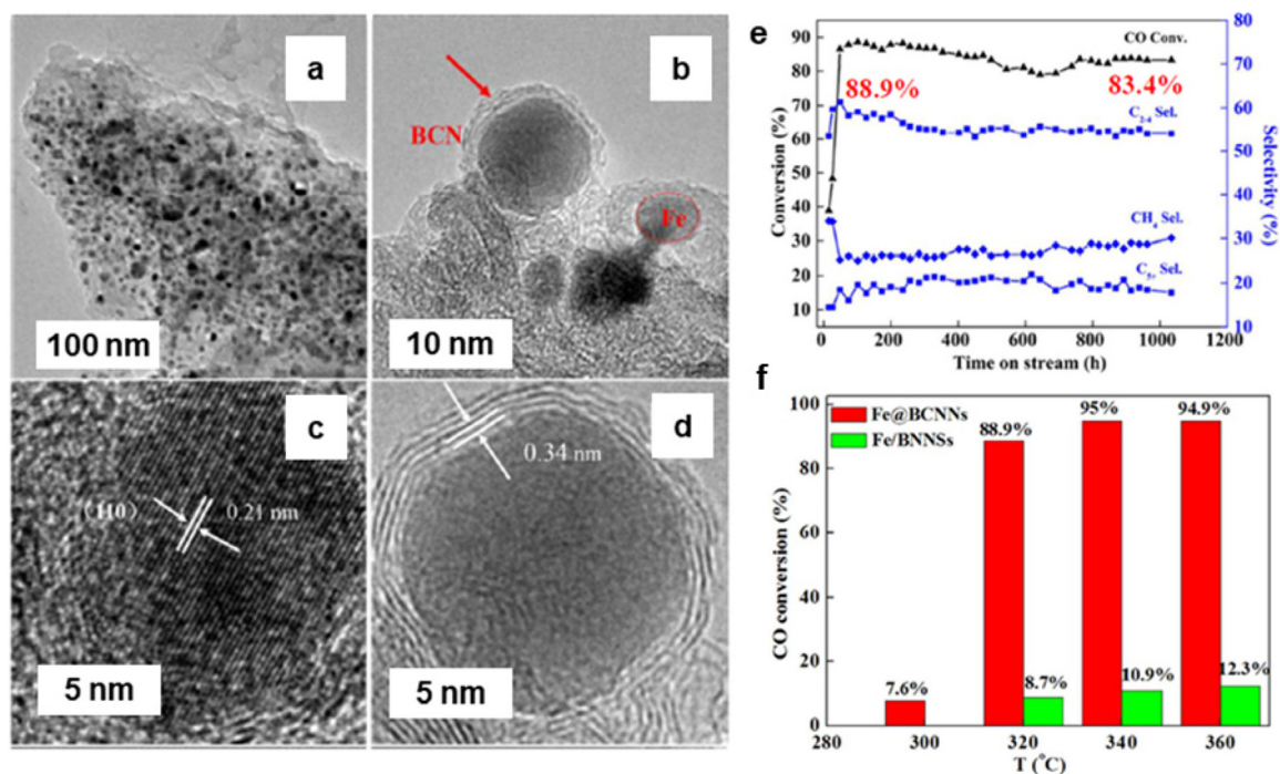
Fig. 42 (a, b) TEM images of Fe@BCNNSs nanocatalyst; (c, d) HR-TEM images of Fe@BCNNSs nanocatalyst; (e, f) Activity of the Fe@BCNNSs nanocatalyst. Reproduced with permission from ref. 263 Copyright 2017, American Chemical Society.
