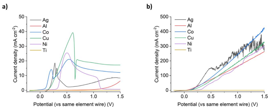
Fig. 1 LSVs of the six metals investigated in \text{ChCl}:2\text{EG} , under (a) silent, and (b) 132\text{ W cm}^{-2} ultrasound. The scan rate was 10\text{ mV s}^{-1} , with a quasi-reference electrode made from the same metal as the metal under investigation. Note 10\times increase in magnitude of Y axis in (b).
