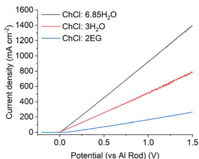
Fig. 3 Linear sweep voltammograms of (a and b) copper, (c and d) cobalt, and (e and f) aluminium disc working electrodes in \text{ChCl}:\text{2EG} and two different \text{ChCl} brines, under (a, c and e) silent, and (b, d and f) 132 \text{ W cm}^{-2} ultrasound. The quasi-reference electrode was the same metal as the working electrode, and the scan rate was 10 \text{ mV s}^{-1} . First scans presented only.
