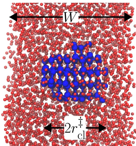
Fig. 2 A snapshot from a seeding simulation with W = 3.5 nm after initial equilibration at T = 220 K, using the mW model. Molecules identified as belonging to the largest ice-like cluster are shown by large blue spheres, while all other molecules are shown by small red spheres. In this case, the initial seed happens to be critical, with approximate radius r_{cl}^* , as indicated.
