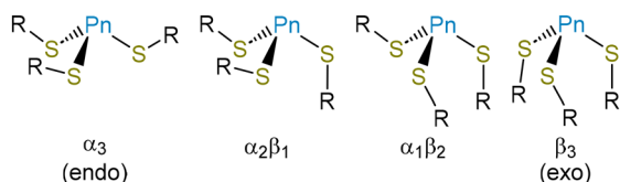
Fig. 2 Schematic depiction of the different conformers of Pn(SR)_3 compounds.
