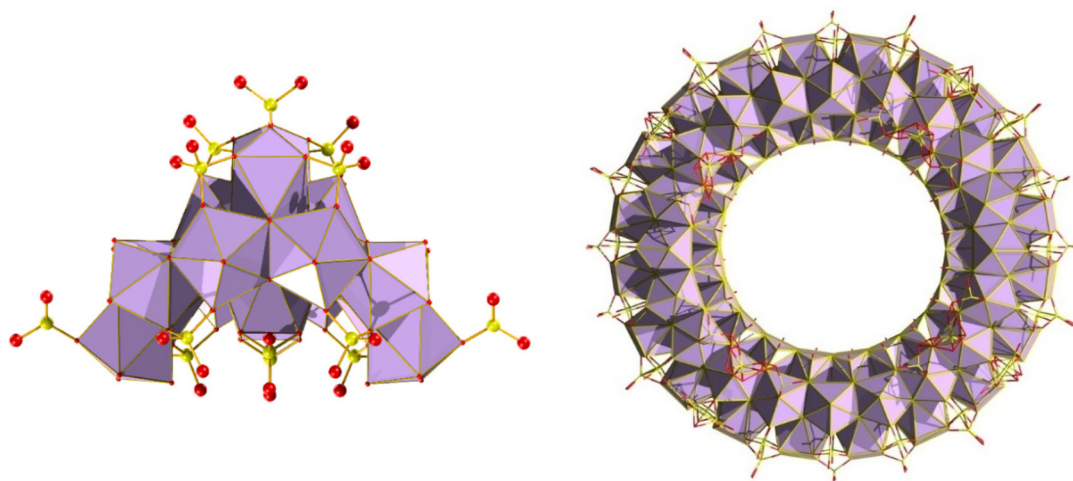
Fig. 24 \text{Zr}_{18} cluster (left), which is isostructural to \text{Hf}_{18} . Lowering sulfate concentration and increasing temperature led to the rearrangement to the toroidal \text{Zr}_{70} cluster (right, top-down view). Colour code: Zr, light purple; S, yellow; O, red. Counter ions and solvate omitted for clarity.
