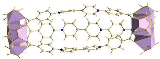
Fig. 23 (\text{Cp}_3\text{Zr}(\mu_3\text{-O})(\mu_2\text{-OH})_3)_2\text{L}_2 , \text{L} = 1,1' -bis(4-carboxyphenyl)-4,4'-bipyridinium dichloride, \text{Cp} = cyclopentadienyl. Colour code: Zr, light purple; C, grey; N, blue; H, white. Counter ions omitted for clarity.
