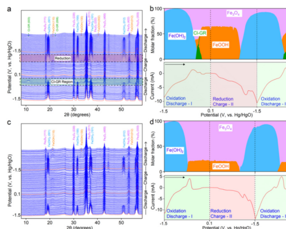
Fig. 8 (a and c) Waterfall plots and (b and d) phase ratio analyses of iron oxides in (a and b) \text{NaOH}/\text{NaCl} and (c and d) \text{NaOH} electrolytes using operando XRD measurements together with cyclic voltammetry at a scan rate of 0.5 \text{ mV s}^{-1} . The selected regions in (a) show the phase transitions during the \text{Cl}^- insertion (discharge) and \text{Fe}(\text{OH})_2 formation (charge). They highlight the XRD patterns depicting the \text{Cl} -GR formation when iron oxides were discharged from -0.42 to -0.18 \text{ V} and the formation of \text{Fe}(\text{OH})_2 when iron oxides were charged from -1.02 to -1.5 \text{ V} , respectively. The X-ray wavelength was corrected to \text{Cu K}\alpha source ( \lambda = 0.15406 \text{ nm} ). Arrows in (b) and (d) indicate the voltage scan direction. Reproduced with permission from ref. 165. Copyright (2023), the American Chemical Society.
