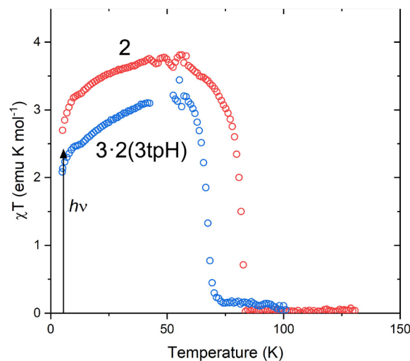
Fig. 5 The LIESST effect in 2 and 3 - 2 (3tpH). After irradiation at 5 K, the temperature was increased at 0.3 \text{ K min}^{-1} . (The noise in the curves at \sim 50 K is due to leakage of oxygen through the fiberoptic sample rod. See Fig. S6 and explanation in the ESI.†)
