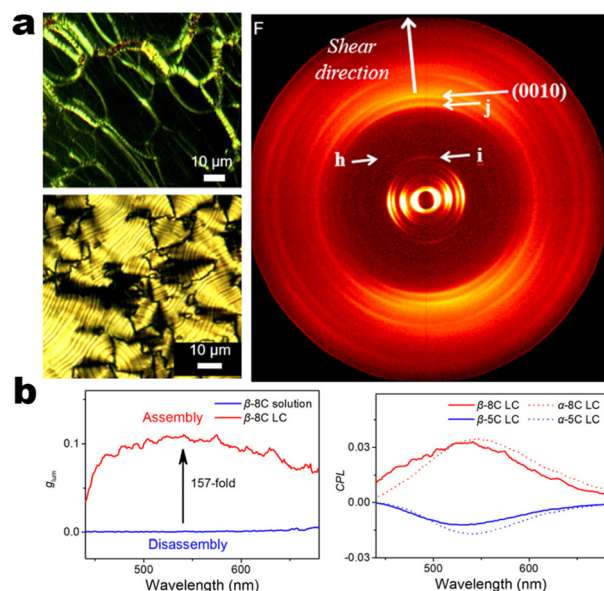
Fig. 13 (a) POM and SAXS images of system 4-9. (b) CPL and g_{lum} spectra of 4-9 films under different states. Reproduced from ref. 104 with permission. Copyright (2020), American Chemical Society.
