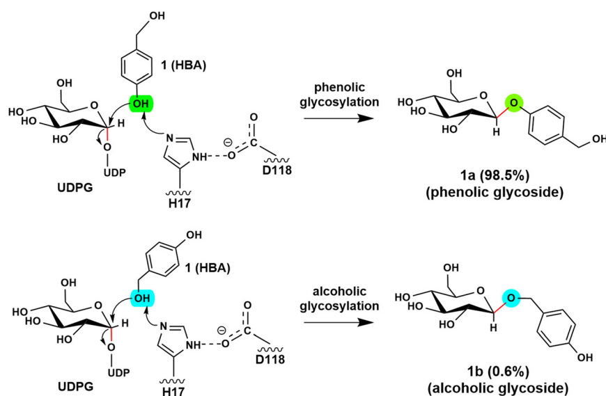
Fig. 1 RrUGT3-catalyzed glycosylation of p -hydroxybenzyl alcohol with high regioselectivity to the phenolic hydroxyl group: phenolic O -glycoside ( 1a ) as the main product (98.5%) and alcoholic O -glycoside ( 1b ) as the minor product (0.6%).
