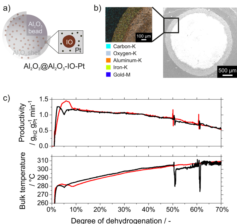
Fig. 3 a) Scheme of the synthesized \text{Al}_2\text{O}_3@/\text{Al}_2\text{O}_3\text{-IO-Pt} catalyst particle consisting of an alumina core and an alumina shell that contains IO supraparticles and is impregnated with Pt. b) SEM image of a cross-section of \text{Al}_2\text{O}_3@/\text{Al}_2\text{O}_3\text{-IO-Pt} and its elemental mapping. c) Productivity (top graph) and bulk temperature (bottom graph) for the dehydrogenation of H18-DBT depending on the DoD in a thermally heated (red) and inductively heated (black) batch experiment using \text{Al}_2\text{O}_3@/\text{Al}_2\text{O}_3\text{-IO-Pt} as the catalyst. Reaction conditions: w_{\text{Pt}} = 0.24 wt%, m_{\text{LOHC}}:m_{\text{Pt}} = 1900 , m_{\text{cat,red}} = 430.0 mg, m_{\text{cat,black}} = 429.0 mg, induction device settings: 273 Oe.
