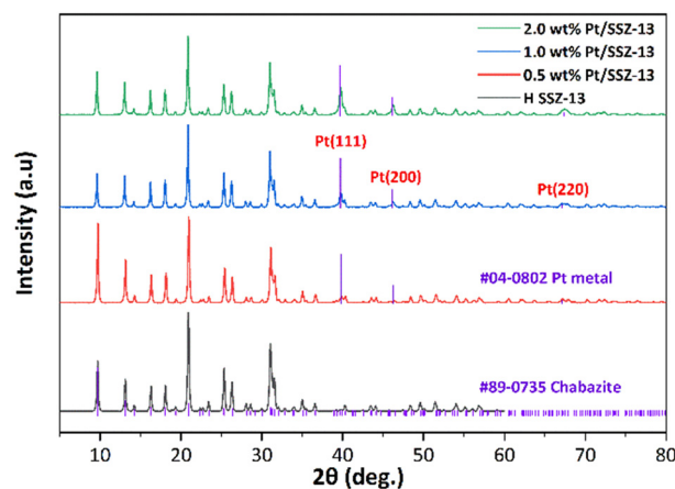
Fig. 1 X-ray diffraction patterns of H-SSZ-13 zeolite and 0.5, 1.0, and 2.0 wt% Pt/SSZ-13 catalysts.
