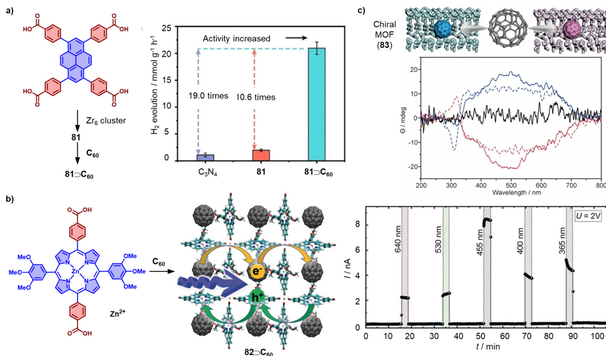
Fig. 33 Selected encapsulations of fullerenes into MOFs to achieve: (a) improved photocatalytic hydrogen evolution, (b) improved photoconduction, (c) chirality transfer from MOF to C 60 . Adapted from ref. 489, 487 and 485 with permission from Wiley-VCH, copyright 2023, 2019, 2021 for (a), (b) and (c), respectively.
