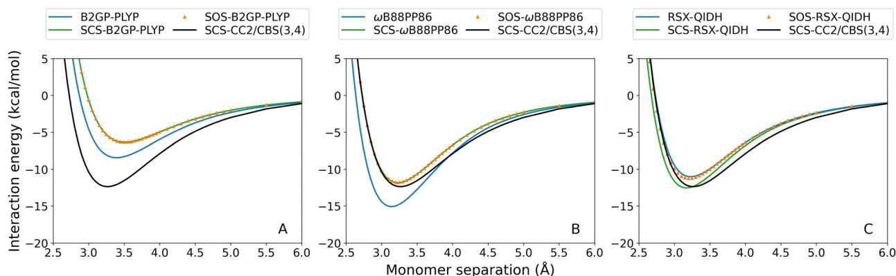
Fig. 8 Toluene-TCNE 3A' dissociation curves for representative TD-DHDFAs and their SCS/SOS variants: (A) B2GP-PLYP; (B) ωB88PP86; (C) RSX-QIDH.
