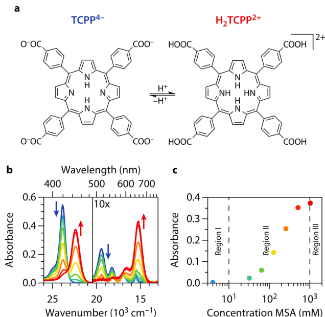
Fig. 1 Steady-state absorption spectroscopy of TCPP and H 2 TCPP 2+ . (a) Molecular structure of carboxylate-form of tetrakis(4-carboxyphenyl)-porphyrin and its fully protonated diacid (TCPP 4- and H 2 TCPP 2+ ). (b) UV/vis spectra of 1.26 μM TCPP 4- in DMF at different acid concentrations from blue to red (0, 4, 32, 64, 128, 256, 512, and 1024 mM MSA). The Soret band (S 0 to S 2 transition) is located at 23.9 × 10 3 cm -1 (419 nm) for TCPP and at 22.4 × 10 3 cm -1 (446 nm) for H 2 TCPP 2+ . The region with the four Q-bands of the porphyrin (lower energy section of the plot) is zoomed in 10 times for visualization purposes. H 2 TCPP 2+ only shows two Q-bands for reasons discussed in the text. (c) Absorbance at 22.4 × 10 3 cm -1 , a direct measure to the amount of H 2 TCPP 2+ , as function of MSA concentration. We indicate three regions, neutral (I), intermediately protonated (II), and fully protonated (III).
