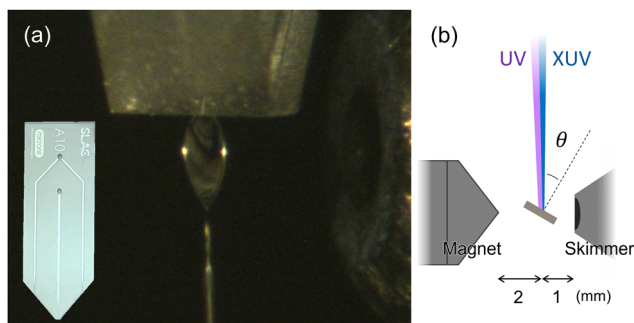
Fig. 1 (a) Photo of gas-dynamic flat jet in operation. Inset shows the flat jet tip (Micronit) used in the experiment. (b) Schematic of the top view of the laser interaction region. The flat jet is ~1 mm away from skimmer with a 500 μm orifice and a magnetic cone is placed ~2 mm away from the jet. The UV/XUV angle of incidence with the jet ( \theta ) is set at 30–60° to optimize photoelectron collection efficiency.
