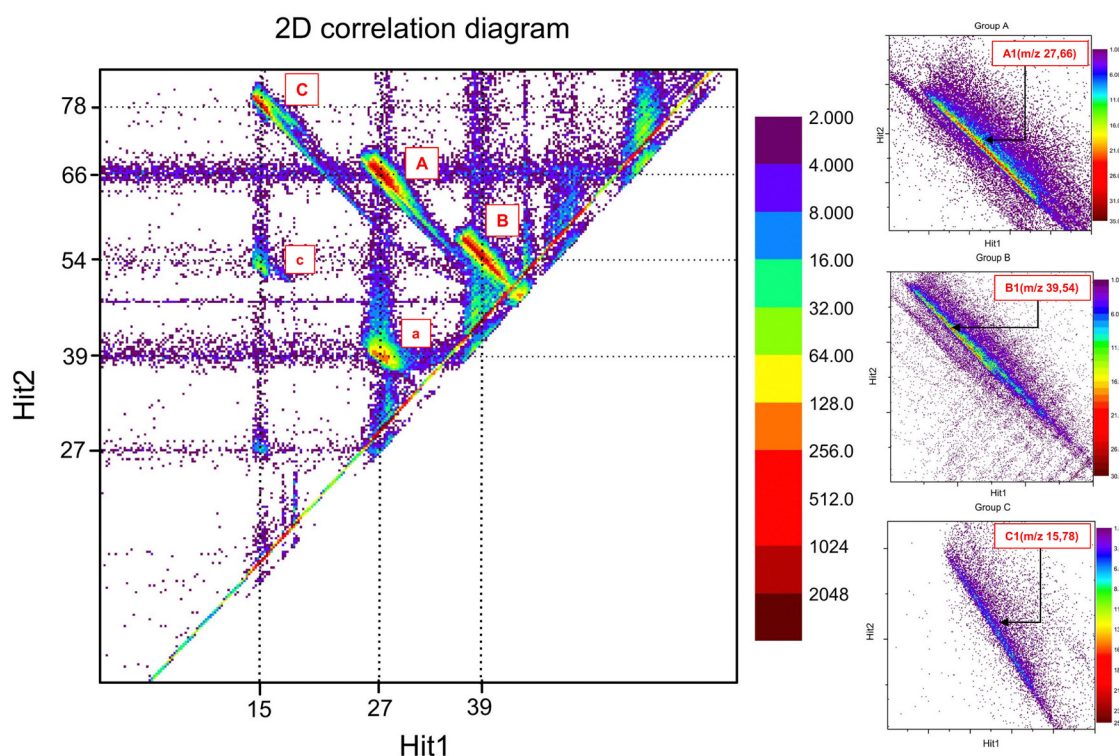
Fig. 2 The ion-ion coincidence diagram of aniline dication. The main channels in the islands with the associated m/z values represented by the dotted lines. An expended view of the islands, which shows the most intense single-step dissociation channels, is shown in the three panels on the right side.
